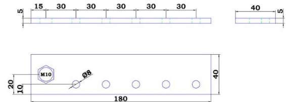
CIP100400060 = Busbar to connect 5 CIP100200100
