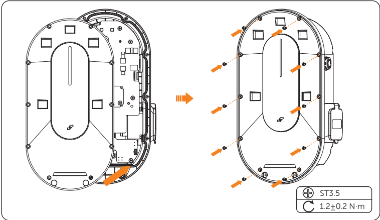
Figure 15-11 Reinstall the front panel cover
