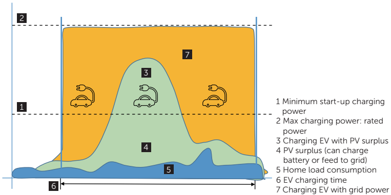
Figure 10-9 Fast mode
