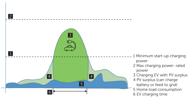
Figure 10-5 Green mode
