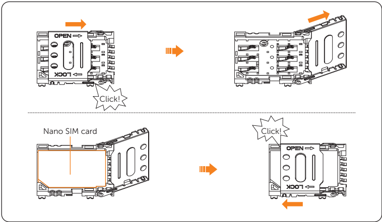
Figure 15-10 Install the SIM card
