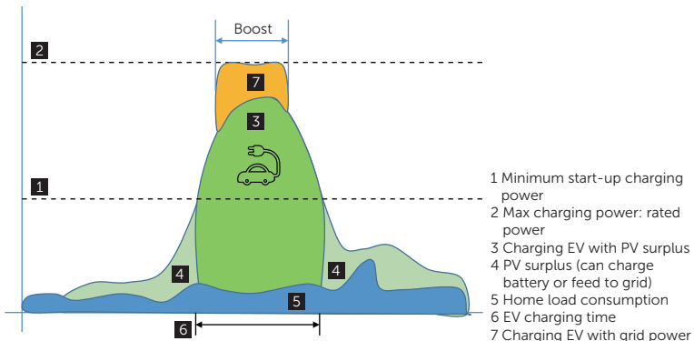
Figure 10-15 Timer Boost
