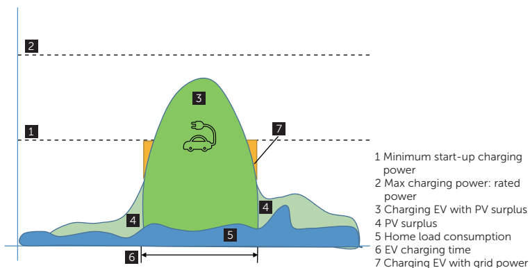
Figure 10-7 Eco mode
