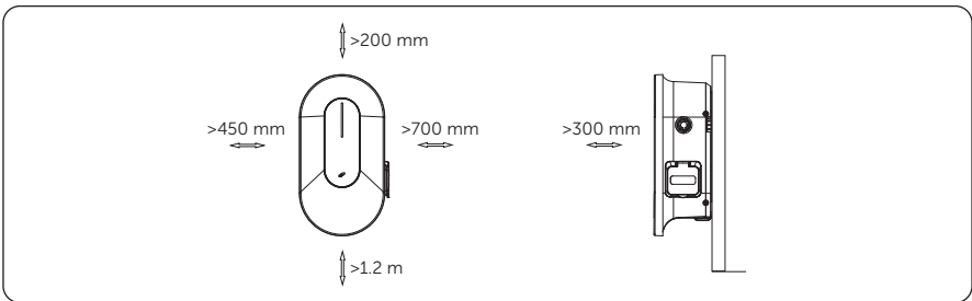
Figure 4-4 Clearance requirement
