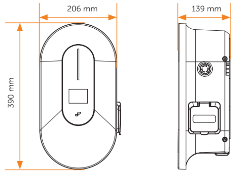
Figure 2-8 Dimensions of Socket Type
