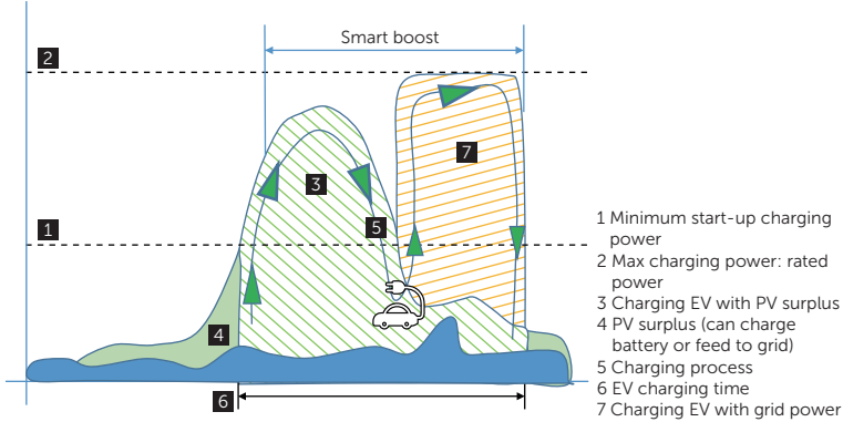
Figure 10-12 Smart Boost
