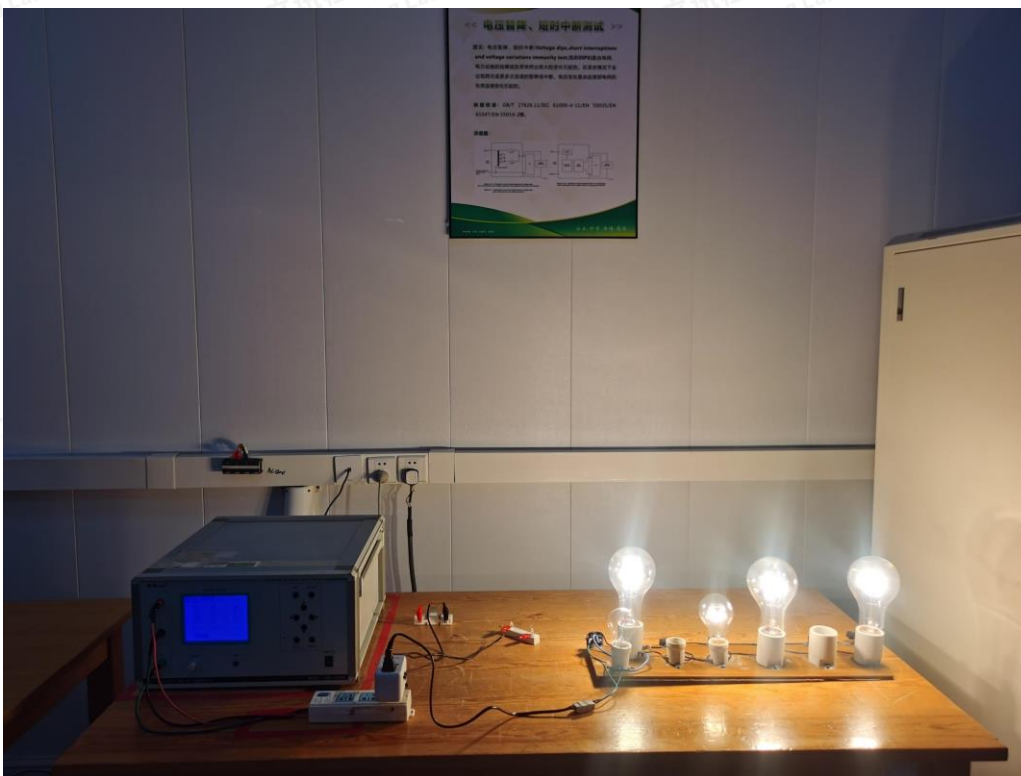
Test Setup Photo of Voltage Dips and Interruptions Test
