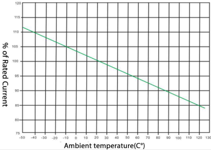
Temperature vs Rate Current
