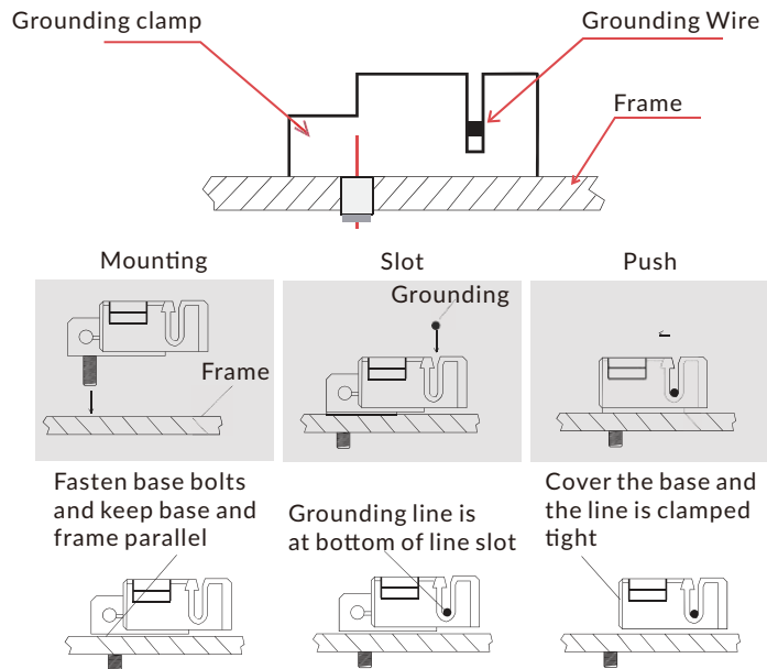
Figure 11 Clamp Grounding Method
