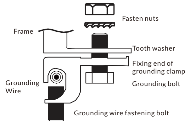
Figure 12 Bolt Grounding Method
